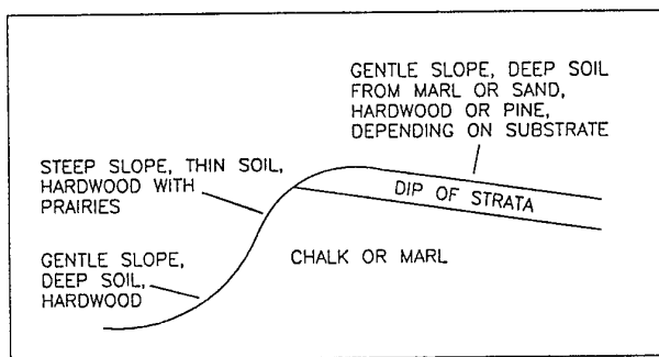
Figure 4. Relationship of forest and prairie to slope, substrate, and soil depth on cuestas.
