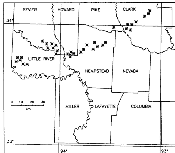
Figure 2. Locations of blackland prairie relicts.
