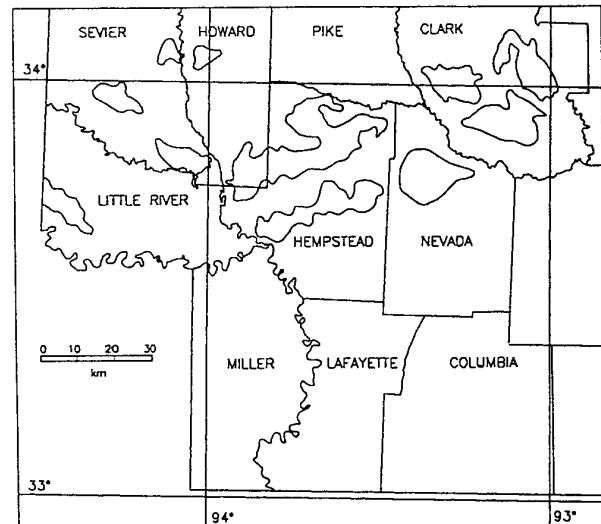
Figure 1. Blackland soil areas (USDA Soil Conservation Service, 1982).
