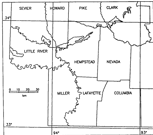
Figure 5. Original distribution of blackland prairies, based on geology, topography, and distribution of relicts.
